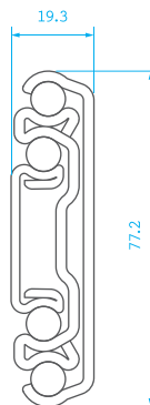
NJ-7J ( 400lbs / 180Kgs )
